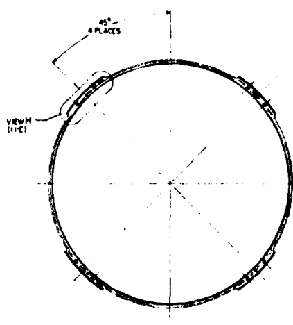
FLANGE A VIEWED FROM INLET END
